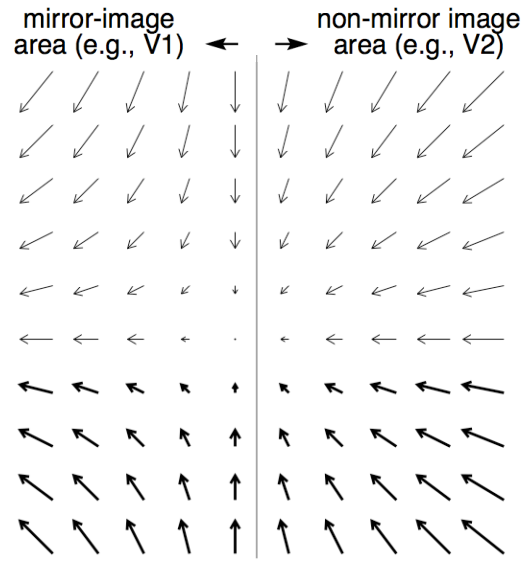
Figure 5. How mirror-image and non-mirror-image areas appear in an arrow diagram. On the left, a mirror-image representation of the left visual field (like right hemisphere V1) is illustrated. It appears as a shear field (arrows tangent to y = mx^{-1} ). On the right, a non-mirror-image representation is illustrated (like V2, but without a split horizontal meridian). It appears, by contrast, as a simple contraction field (arrows along y = mx ).
