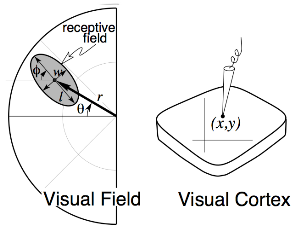
Figure 1. Seven receptive field parameters. The location of the recording site is measured from the penetration photograph (x, y) , the center of the receptive field is defined by its eccentricity and angle (r, \theta) , and the receptive field shape is parameterized by the length, width, and angle of the best-fitting ellipse (l, w, \phi) . An arrow diagram (see Figs. 5, 6) is constructed by placing a sealed copy of the arrow from the center of gaze to the receptive field center (thick arrow) at the x, y -position on the cortex from which that receptive field was recorded. A receptive field on the horizontal meridian of the left hemifield is conventionally labeled with an angle of 0^\circ .
