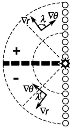
Figure 11. The local visual field sign is determined by measuring the (clockwise) angle, \lambda , between the eccentricity gradient (direction of \nabla r ), and the receptive field polar angle gradient (direction of \nabla \theta ). An angle of approximately 90^\circ ( 0 < \lambda < \pi ) signifies a non-mirror-image mapping of the contralateral (left) hemifield while an angle of approximately 270^\circ ( \pi < \lambda < 2\pi ) signifies a mirror-image mapping of the same hemifield. This is a robust, relative local measure capable of distinguishing non-mirror-image from mirror-image regions that is invariant to rotation and distortion of local map regions. Visual field sign is also invariant to receptive field coordinate transformations; to compute it, only the relative position of receptive fields must be known.
