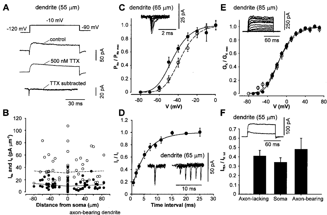
patches in both cases). G_{\text{K}} , \text{K}^+ conductance; G_{\text{K max}} , maximal \text{K}^+ conductance. Inset shows corresponding \text{K}^+ outward currents in dendritic outside-out patch. Data were fitted with Boltzmann functions raised to the fourth power (midpoint potentials are -15.3 and -15.6 \text{ mV} , respectively). (F) Effect of 10 mM TEA on patches from the axon-lacking dendrite, soma, and axon-bearing dendrite (5, 6, and 8 patches, respectively). The 100-ms pulses are to 70 \text{ mV} . I_{\text{TEA}} , peak \text{K}^+ current in the presence of TEA; I_{\text{K tot}} , total \text{K}^+ current in control conditions. The ratio of steady state to peak current was 0.75 \pm 0.05 (dendrite) and 0.66 \pm 0.07 (soma) in the control and 0.52 \pm 0.07 (dendrite) and 0.48 \pm 0.12 (soma) in 10 mM TEA.
