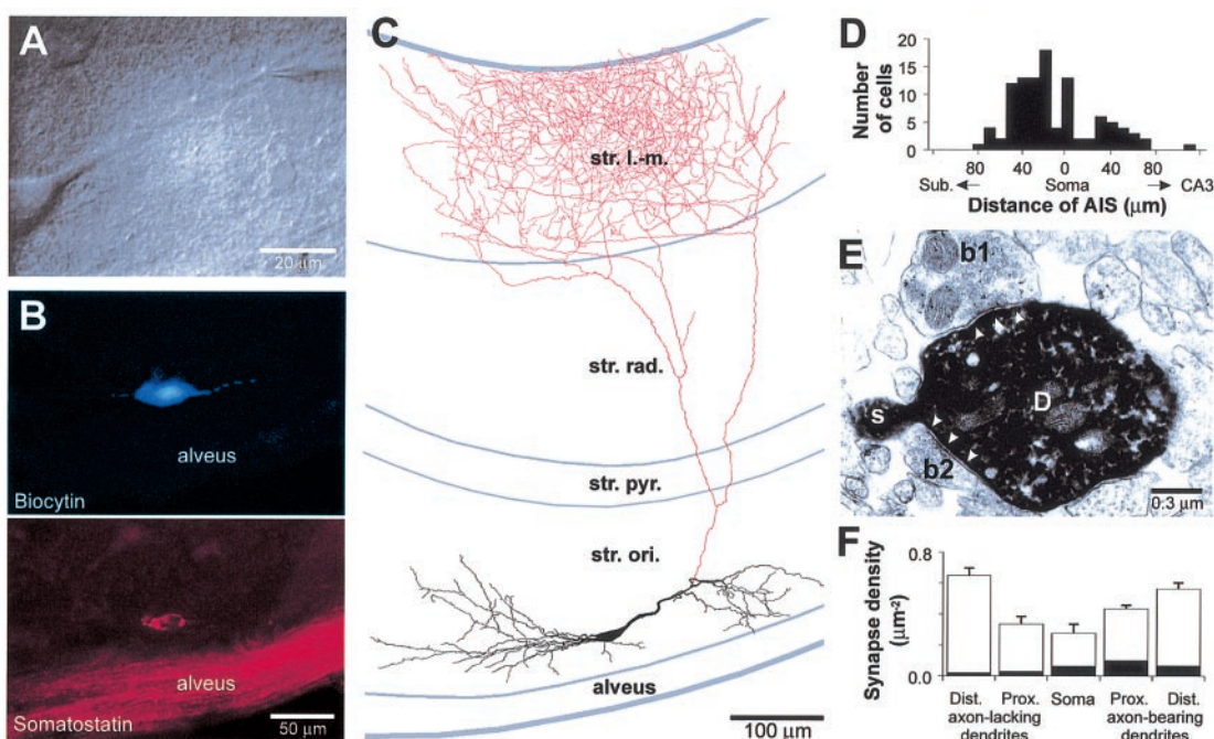
bars, two cells) on five selected regions of oriens-alveus interneurons. Distal dendrites are \geq 100 \mu\text{m} from the soma, and proximal dendrites are \leq 65 \mu\text{m} from the soma. Error bars represent SEM.
