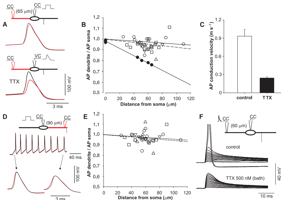
Fig. 4. Active somatodendritic propagation of action potentials and boosting of EPSPs. (A) Active and passive action potential propagation in the same oriens-alveus interneuron. Upper traces, dendritic (red) and somatic (black) action potential evoked by a current pulse (40 ms, 200 pA applied at the soma); lower traces, dendritic response evoked by the previously recorded somatic action potential used as a voltage-clamp (VC) command in the presence of 500 nM TTX. (B) Ratio of dendritic and somatic action potential (AP) amplitudes plotted versus the distance from the soma for the axon-bearing dendrite (open circles and continuous line at 22° to 25°C; triangles at 33° to 36°C) and the axon-lacking dendrite (squares and dashed line at 22° to 25°C; inverted triangles at 33° to 36°C). In the control, the ratio is close to unity, almost independent of location. In TTX, the ratio is smaller than unity and decreases with distance (solid circles and lower continuous line at 22° to 25°C). Points at a distance of 0 μm represent double-soma recordings. Mean somatic action potential amplitude is 115 \pm 2 mV at 22° to 25°C and 98 \pm 3 mV at 33° to 36°C. (C) Conduction velocities in active (open bar, 21 cells) and passive dendrites (solid bar, 4 cells), determined from the time difference between the peaks of action potentials at two sites or from the time difference between the peaks of the somatic voltage-clamp command and the dendritic response, respectively. For the active conduction velocity, a subset of cells in which the axon originated outside the two recording sites was analyzed. Error bars represent SEM. (D) Somatodendritic action potential propagation during a spike train. Lower traces are expanded versions of the first and the last action potential in the train, recorded simultaneously at the dendrite and the soma (100-ms,
